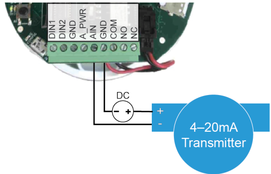
Sensor powered by external source
