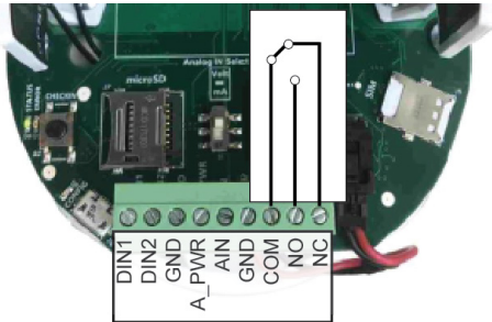
Relay de-energized (COM connected to a NC)
