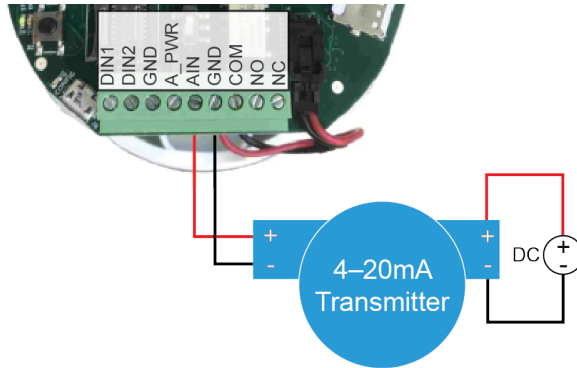
Sensor Setup in Active Loop
