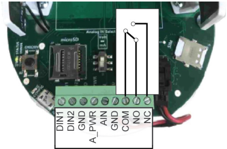
Relay energized (COM connected to NO)
