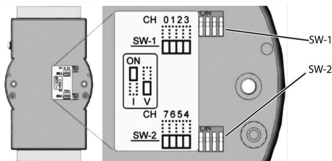
Cut-outs providing access to SW-1 and SW-2 and an illustration map on the back of the Analog Input Expansion Module
