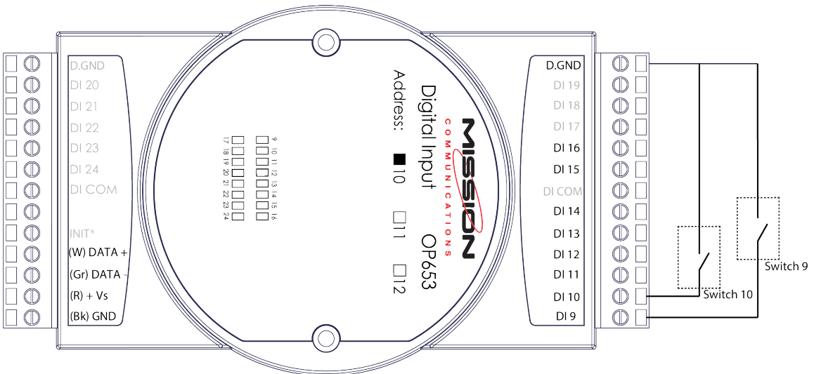
Figure 8: Dry Contact Wiring Diagram Logic level 1: close to GND, Logic level 0: open
