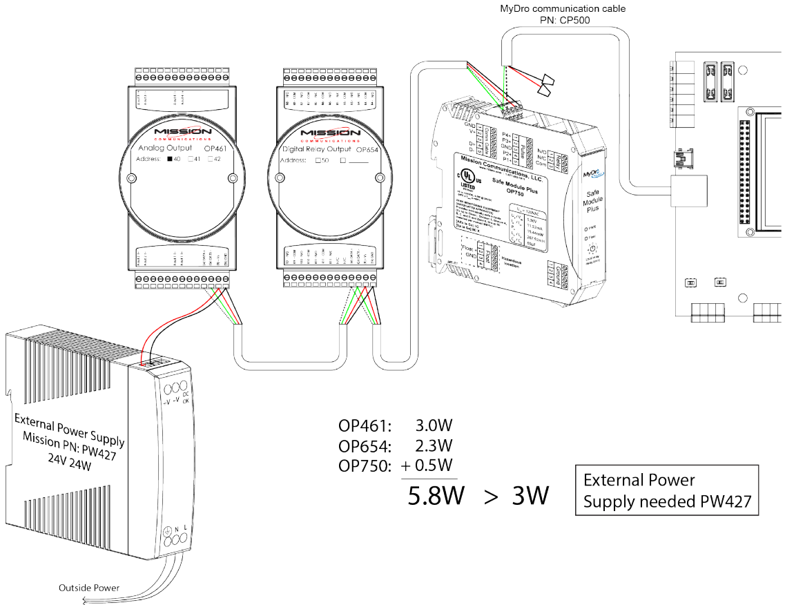
Figure 11: Multiple module network powered by external supply. Cap the power ends (red, black) of the communications cable to avoid a short.
