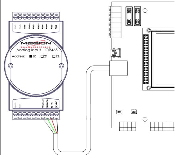
Figure 1B: Other Expansion Modules
