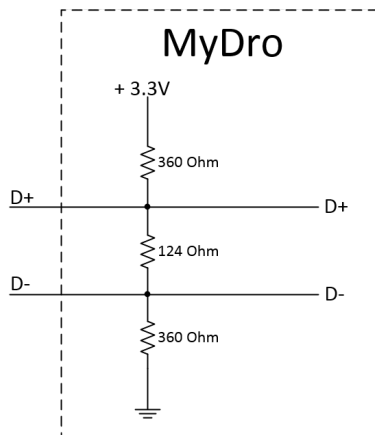
Figure 12: RS485 impedance characteristic internal to the MyDro
