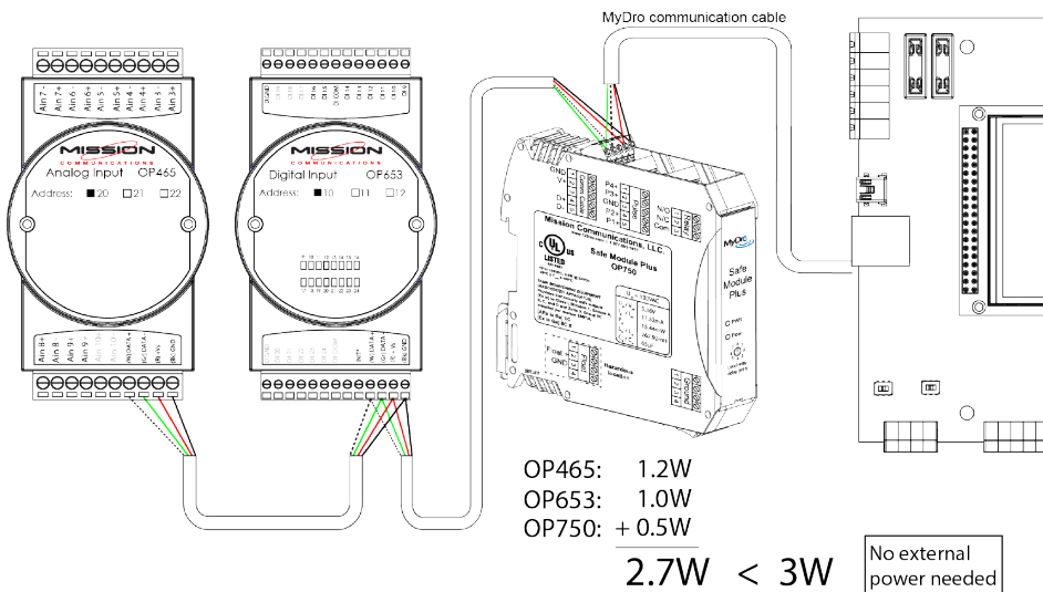
Figure 10: Multiple module network powered by communications cable
